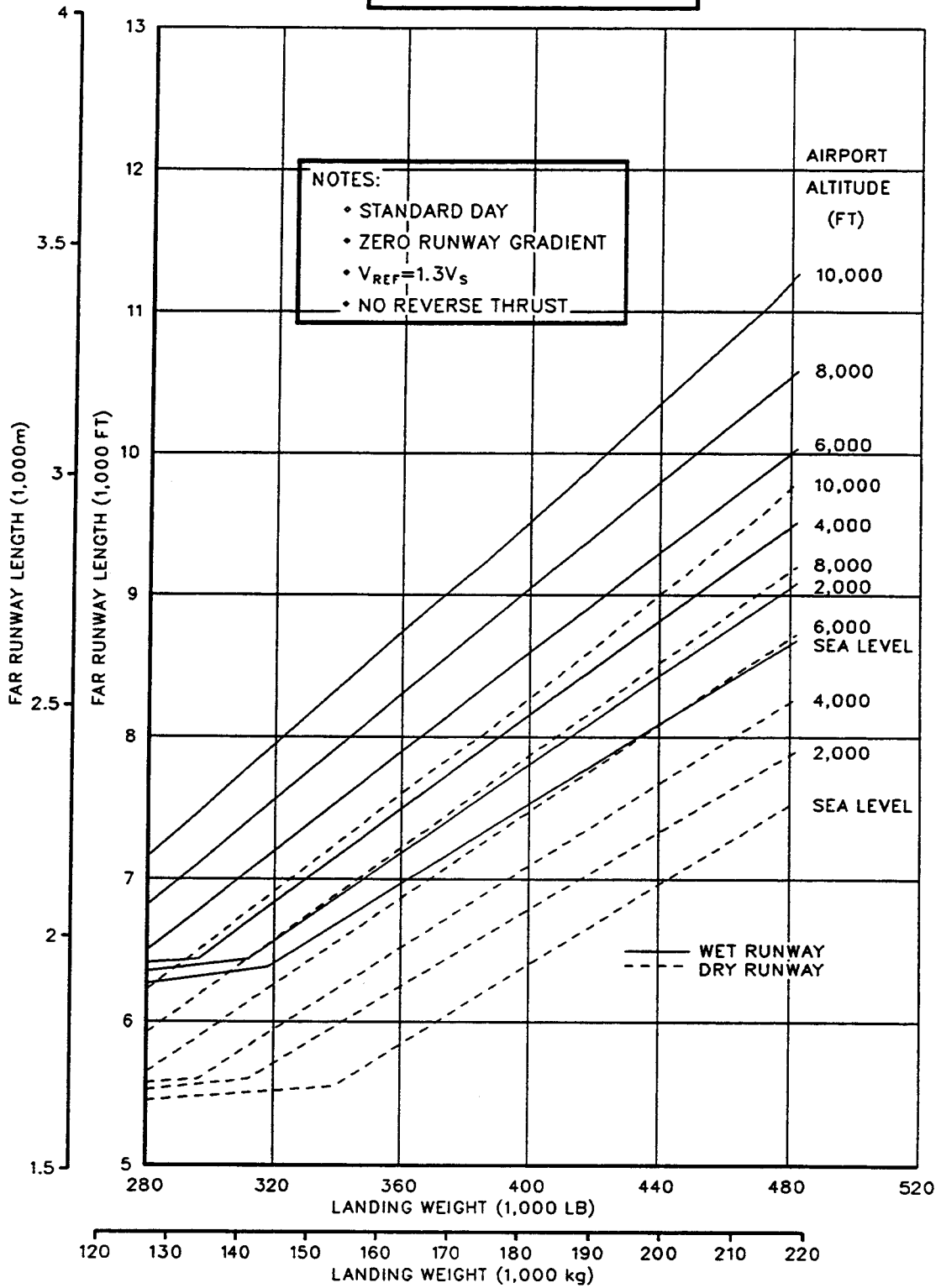
FAR LANDING RUNWAY LENGTH REQUIREMENTS FLAPS 50 DEGREES MODEL MD-11
