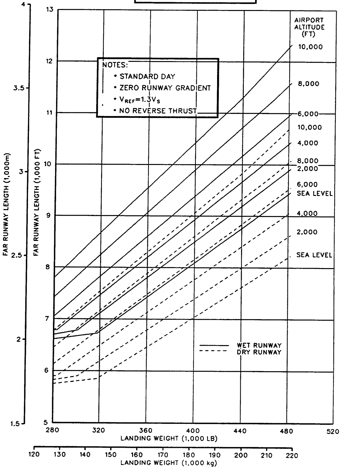
FAR LANDING RUNWAY LENGTH REQUIREMENTS FLAPS 35 DEGREES MODEL MD-11
